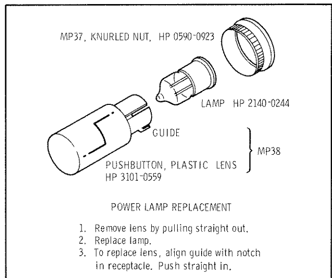
Figure 3-1. Lamp Replacement
